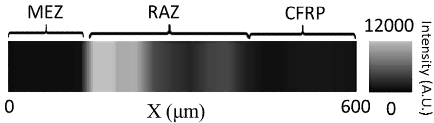
図Ⅲ2.1-35 Mapping of Raman shift at the wavenumber of 2000 \text{cm}^{-1} from kerf to distance of 600 \mu\text{m} on CFRP after laser irradiation
