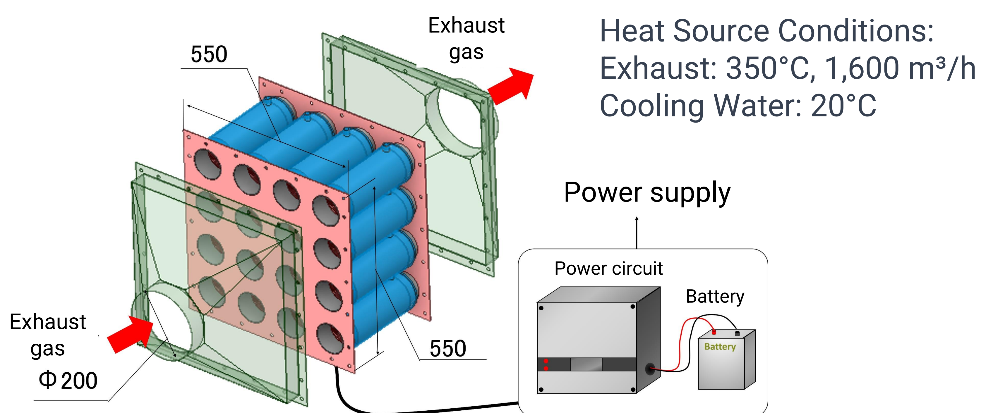
A Power Generation System(1.5 kW) with Parallel connected ' Thermo-Electric Power Tubes'.
