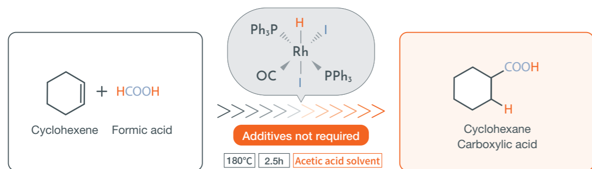
Using acetic acid as solvent, carboxylic acid obtained in high yields without using additives.
