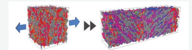
Calculation of uniaxial elongation using coarse-grained molecular dynamics
