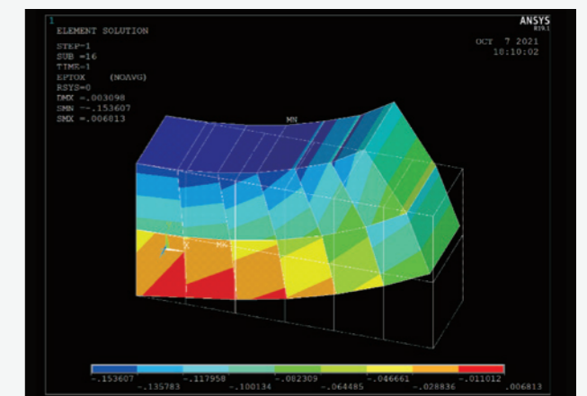
The results of finite element analyses confirm that the predicted level of deformation is attained when electric fields are applied.
