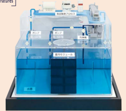
Model of high-density thermal energy storage system applied to food production process
