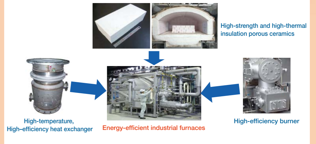
Thermal management system for energy-efficient industrial furnaces
