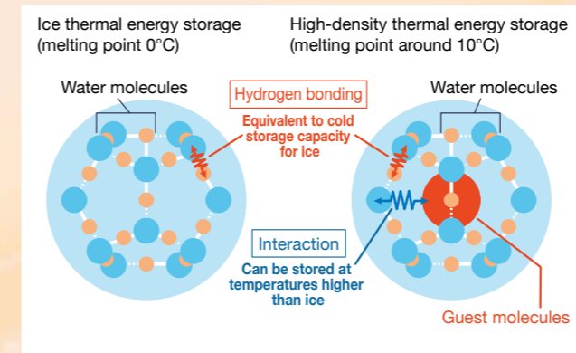
Clathrate hydrates with guest materials encapsulated in caged structure of water molecules
