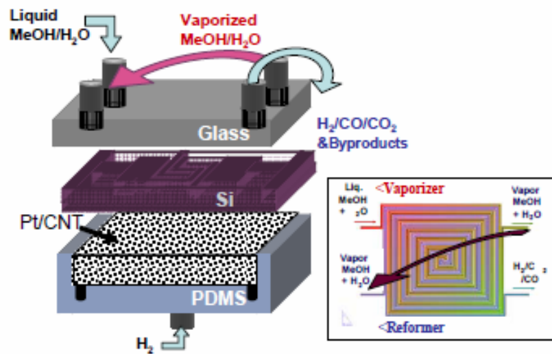
Figure 2. Schematic view of the proposed methanol steam reforming system
