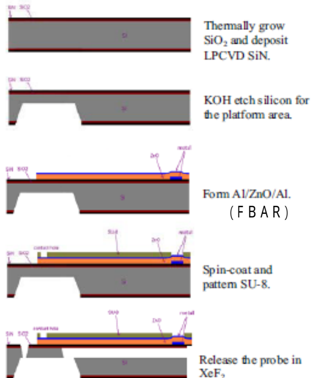
Fig. 5. Fabrication steps of an SU-8 probe integrated with an FBAR sensor.
