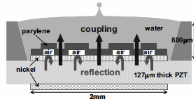
Fig. 1. Cross-sectional view of the ejector with the acoustic lens employing air-reflectors.
