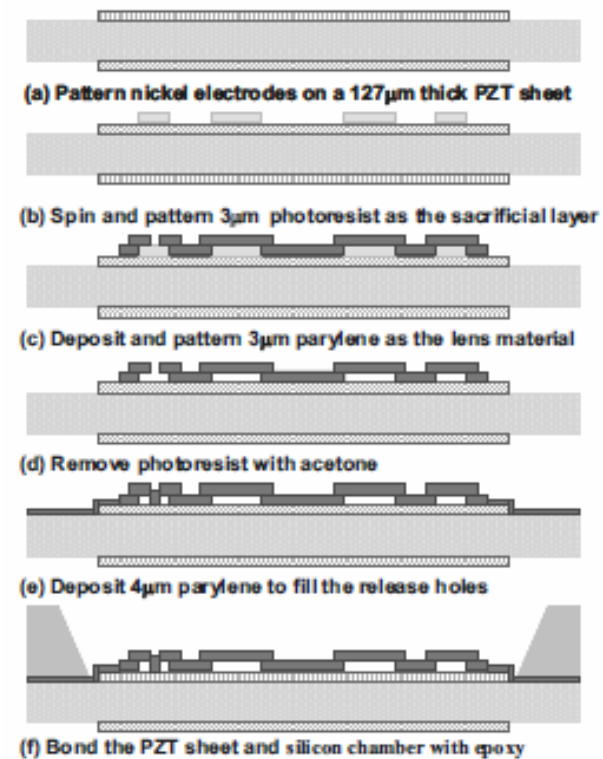
Fig. 3. Brief fabrication steps.
