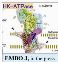
HK-ATPase \alpha -subunit EMBO J, in the press PNAS, 104, 10034-10039 (2007) Nature, 458, 597-602 (2009) by X-ray
