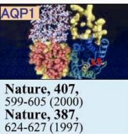
AQP1 Nature, 407, 599-605 (2000) Nature, 387, 624-627 (1997) bR Nature, 389, 206-211 (1997)
