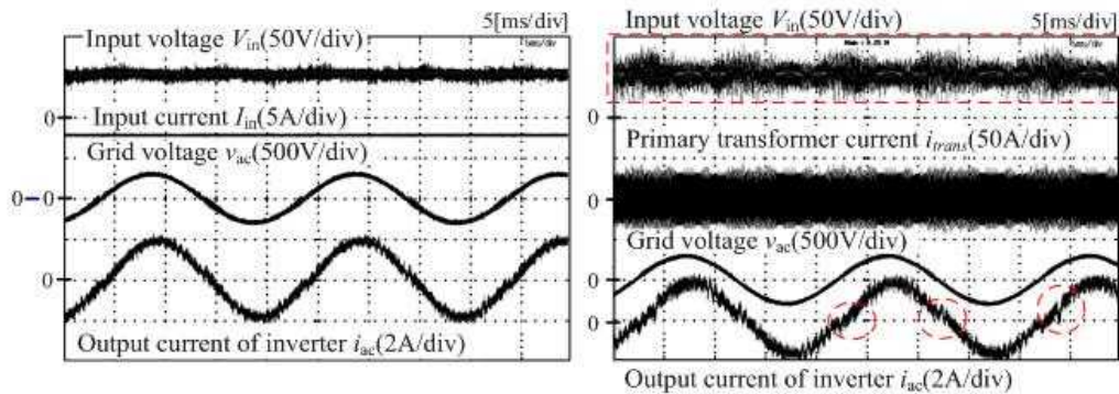
(a) PDM 適用前
