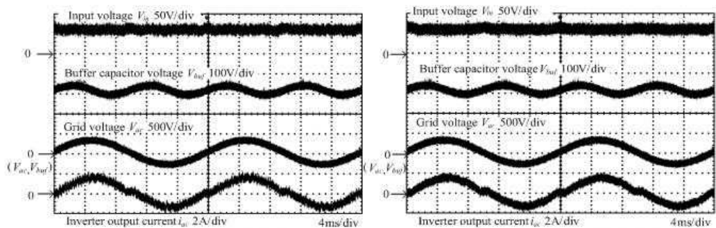
(a) 従来変調(PWM_PDM)
