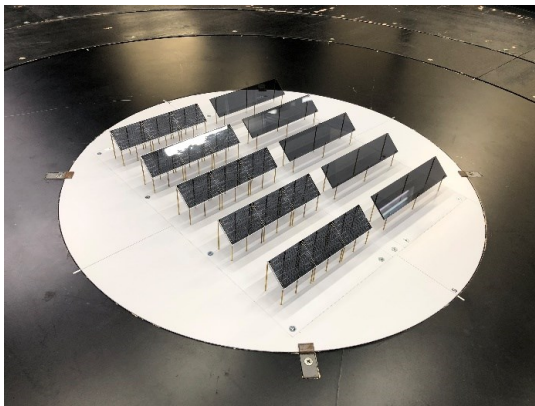
(c) m40h3s(h=3m, d=3m , \theta = 40 度)
