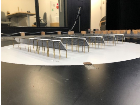
(a) m50h2(h=2m , \theta = 50 度)
