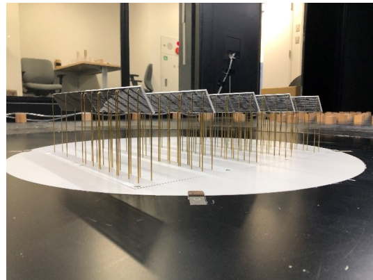
(e) m60h9(h=9m, \theta = 60 度)
