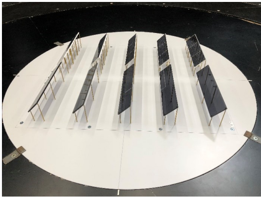
(c) m45h3s(h=3m, d=3m, \theta = 45 度)
