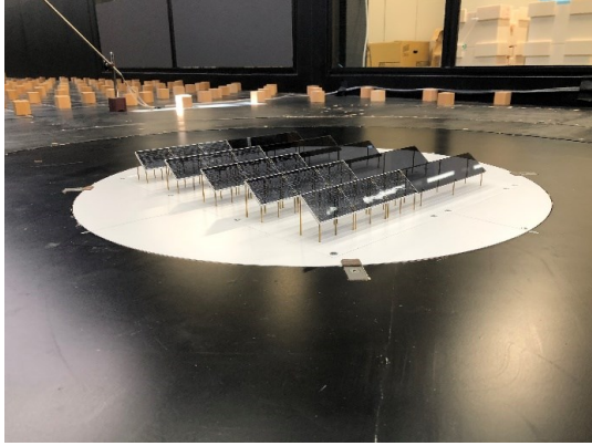
(a) m40h2(h=2m , \theta = 40 度)
