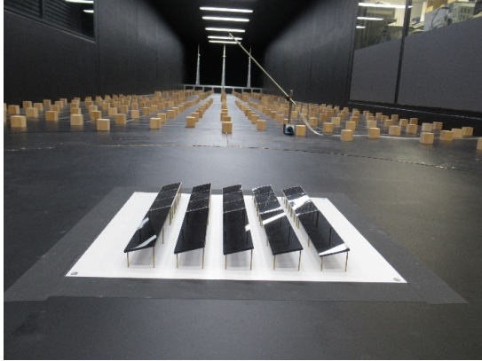
(a) m15h2( h=2\text{m} , \theta =15^\circ )
