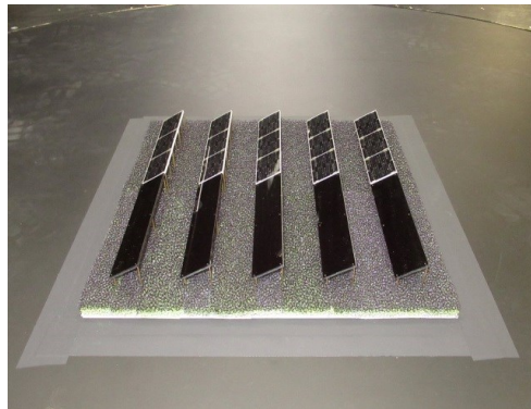
(g)群配置 (m30h3c2 植栽 2m)
