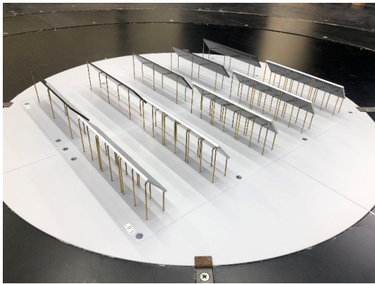
(c) m50h3s(h=5m, d=3m, \theta = 50 度)
