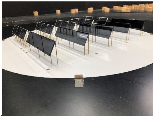
(c) m60h3s(h=3m, d=3m , \theta = 60 度)
