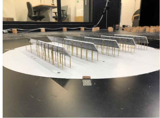
(b) m50h3(h=3m , \theta = 50 度)
