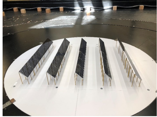
(b) m45h3(h=3m , \theta = 45 度)
