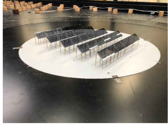
(b) m40h3(h=3m , \theta = 40 度)
