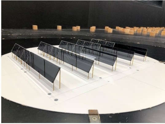
(a) m60h2(h=2m , \theta = 60 度)
