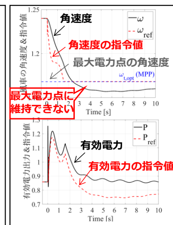
Case 3(Droop)
