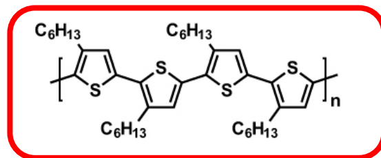
P3HT(Poly(3-hexylthiophene-2,5-diyl))
